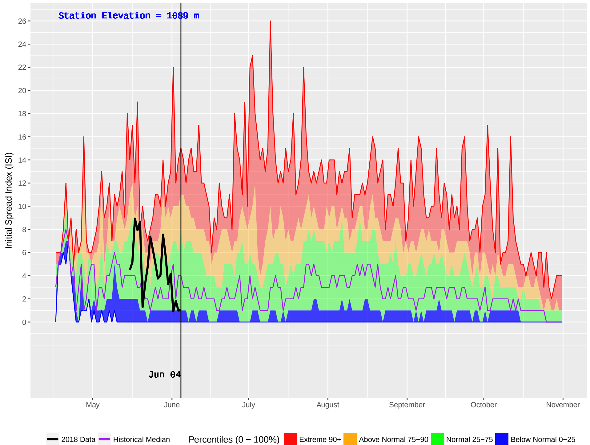
EAST OOTSA (170) : Historical (1986–2016) and Current (2018) Noon Initial Spread Index (ISI)
