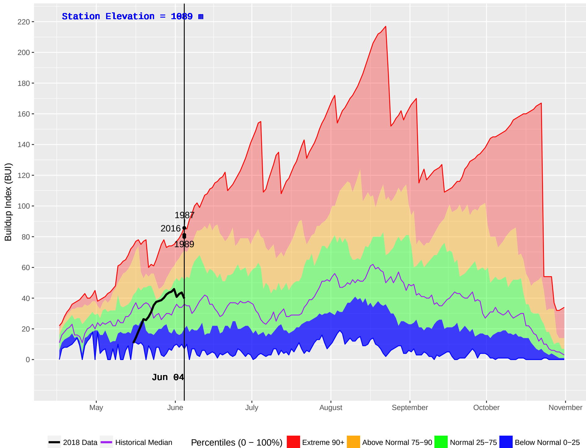
EAST OOTSA (170) : Historical (1986–2016) and Current (2018) Noon Buildup Index (BUI)
