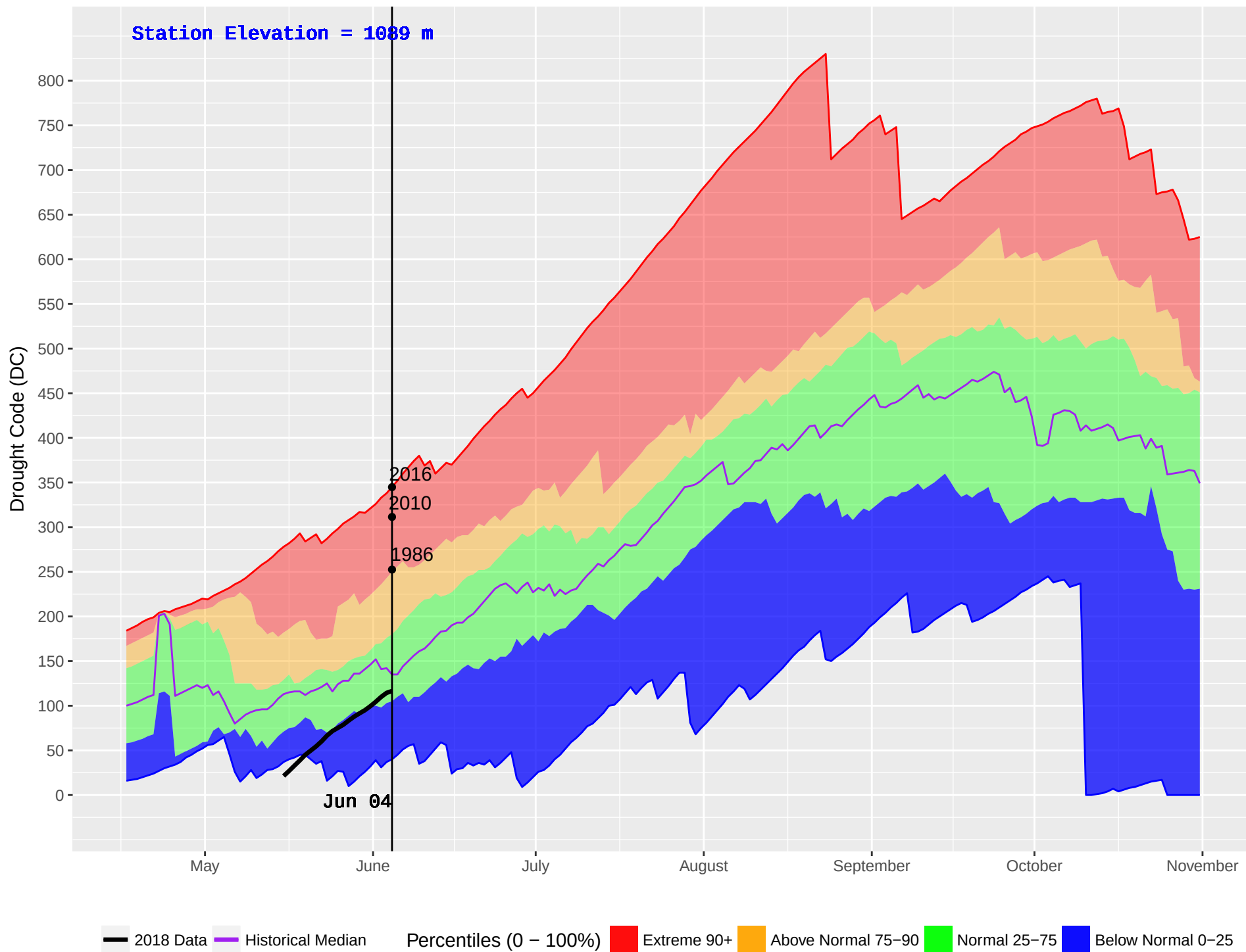
EAST OOTSA (170) : Historical (1986–2016) and Current (2018) Noon Drought Code (DC)
