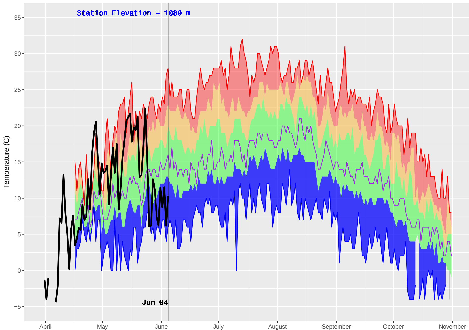
EAST OOTSA (170) : Historical (1986–2016) and Current (2018) Noon Temperature
