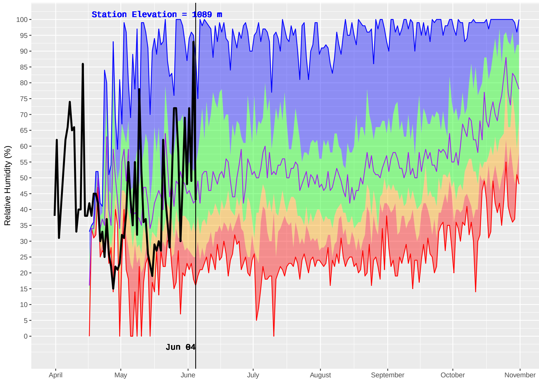
EAST OOTSA (170) : Historical (1986–2016) and Current (2018) Noon Relative Humidity
