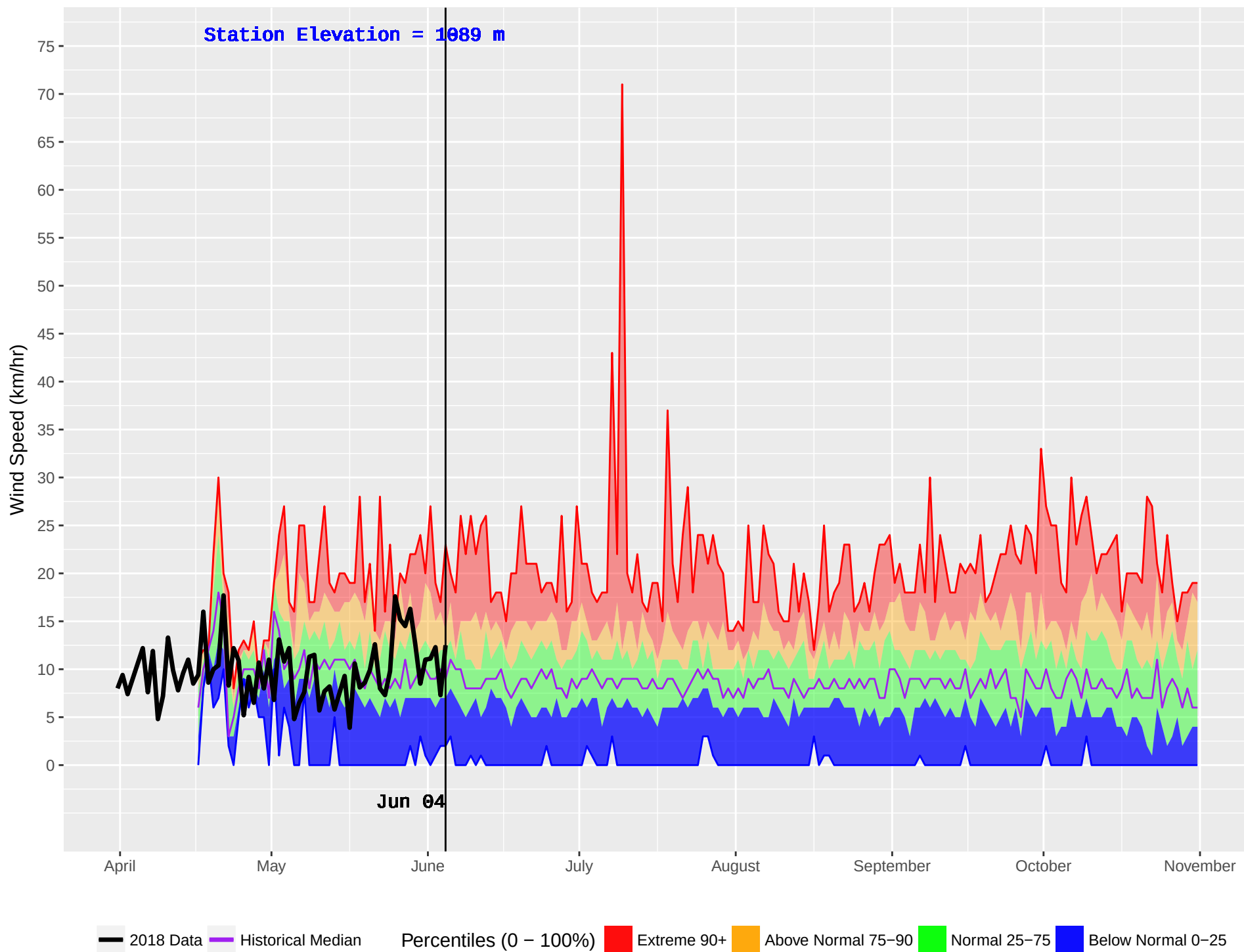
EAST OOTSA (170) : Historical (1986–2016) and Current (2018) Noon Wind Speed
