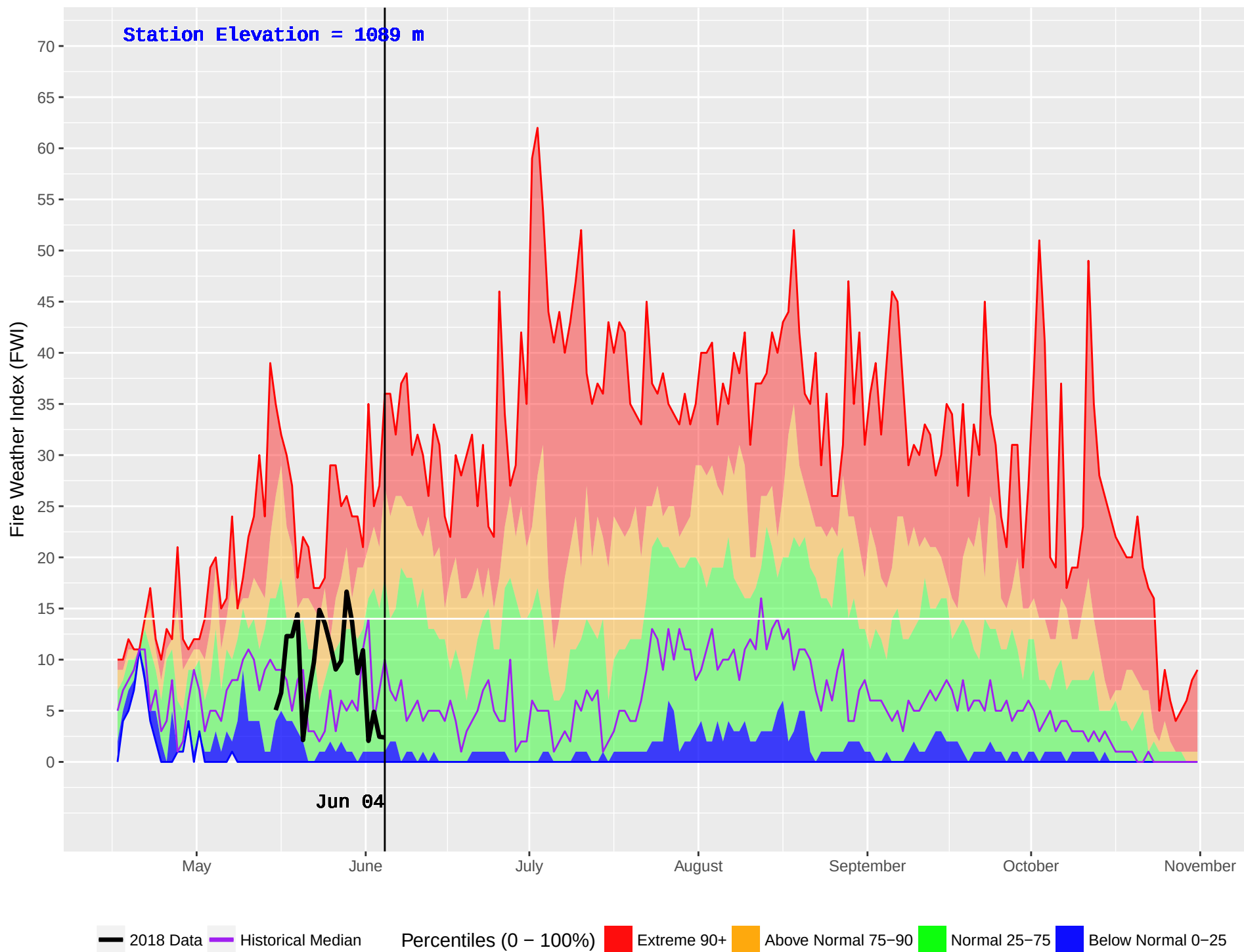
EAST OOTSA (170) : Historical (1986–2016) and Current (2018) Noon Fire Weather Index (FWI)
