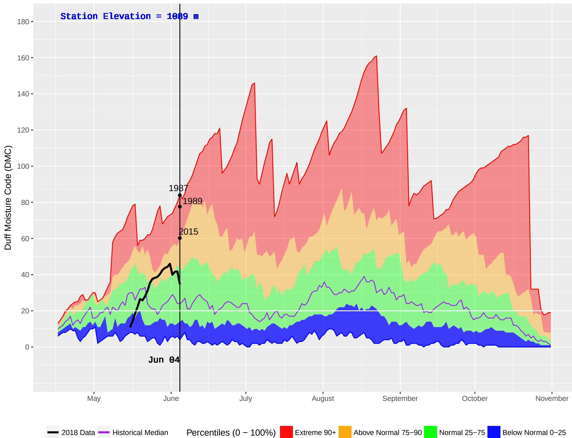
EAST OOTSA (170) : Historical (1986–2016) and Current (2018) Noon Duff Moisture Code (DMC)
